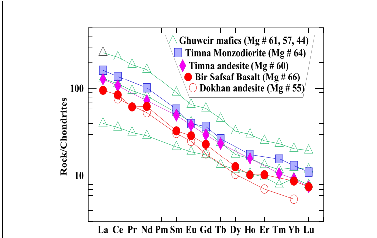
Figure 3. Chondrite-normalized Patterns for the Ghuweir Mafics and the Equivalent Rocks from the Adjacent Countries. The Mg #s are Calculated According to the Formula Mg \# = \frac{\text{mol. prop. Mg}}{\text{mol. prop. Mg} + \text{mol. prop. Fe}} \times 100 .
